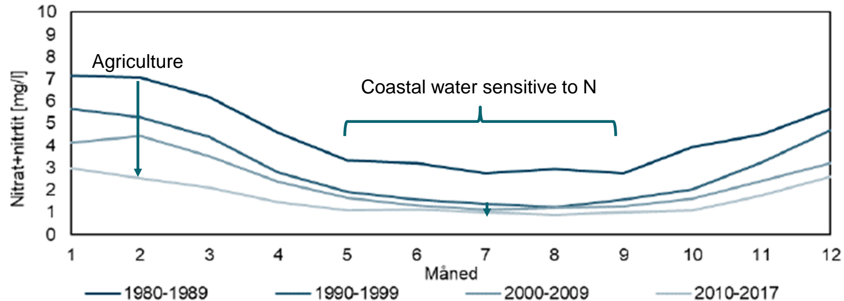
Nitrate concentration in stream
